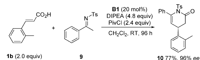
Scheme 3. Reaction with the acyclic imine 9.
